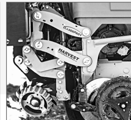
LASERPRO1 + integrated LASERSWEEP™ row cleaner Integrated X-plate mount with no in-field row unit interference
